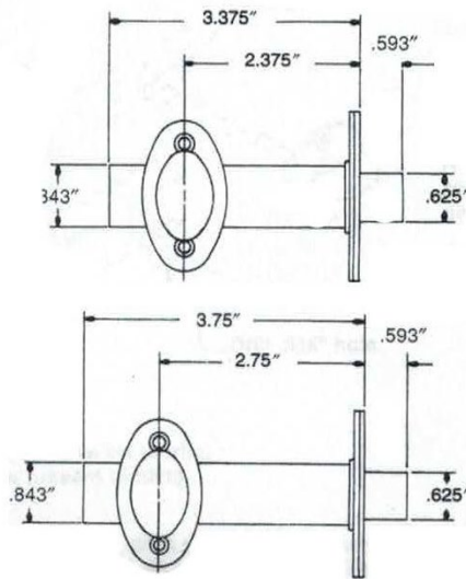
Hub: for 7 x 7 mm spindle
