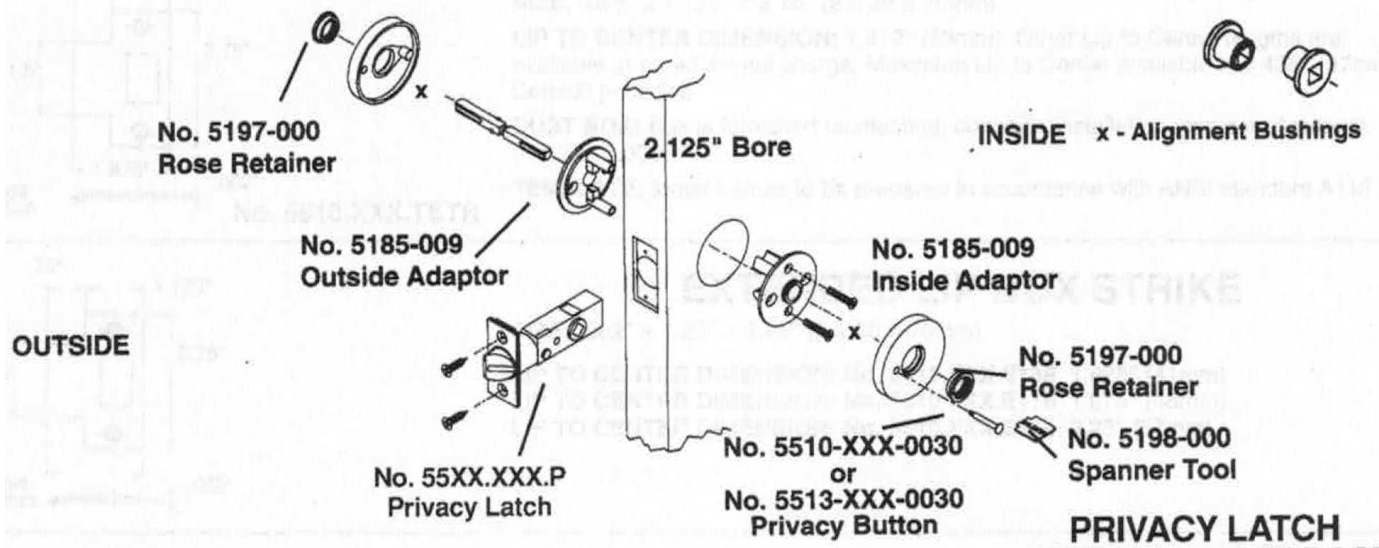
PRIVACY DIAGRAM SETUP US
