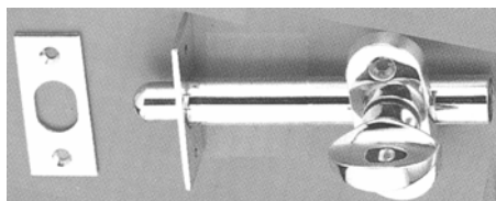
Privacy turning bolt #18.017 with oblong escutcheon thumb-turn inside, indicator outside.
