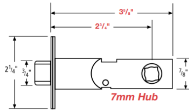
Hub: for 7 x 7 mm spindle
