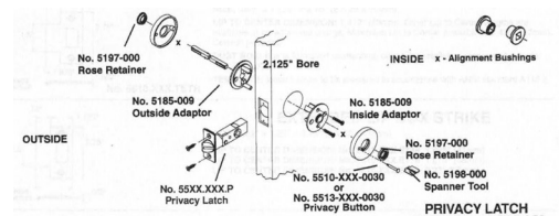
Privacy diagram USA
