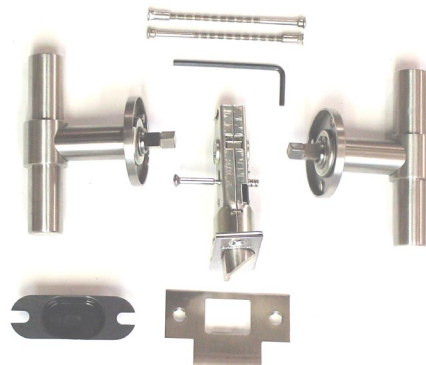
Privacy set up diagram Euro levers
