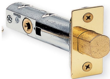
18.455 Privacy Bolt 065/238 with 2 3/8 inch backset
