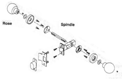
Passage setup diagram
